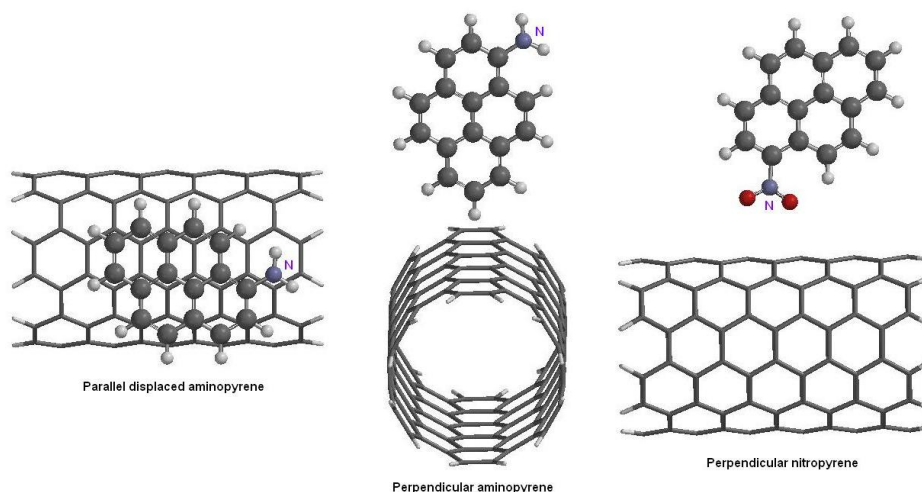
Figure 1. Parallel and perpendicular orientations of aminopyrene and nitropyrene relative to a (6, 6) CNT surface.
